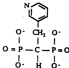
Risedronate
